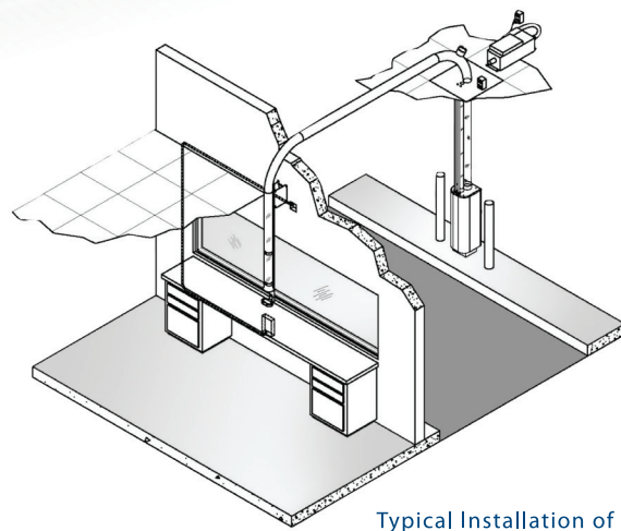
Typical Installation of Integrated 522 System
